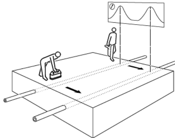
Figure 5.5: Inductive search
