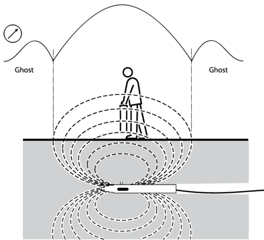
Figure 8.9 Locating a sonde
