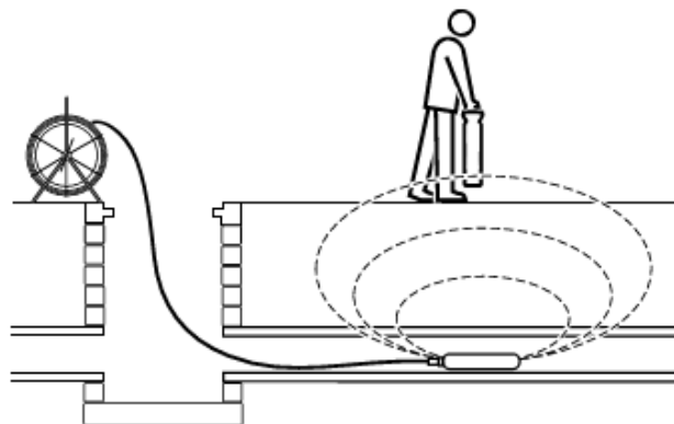
Figure 8.8 Sonde deployment
