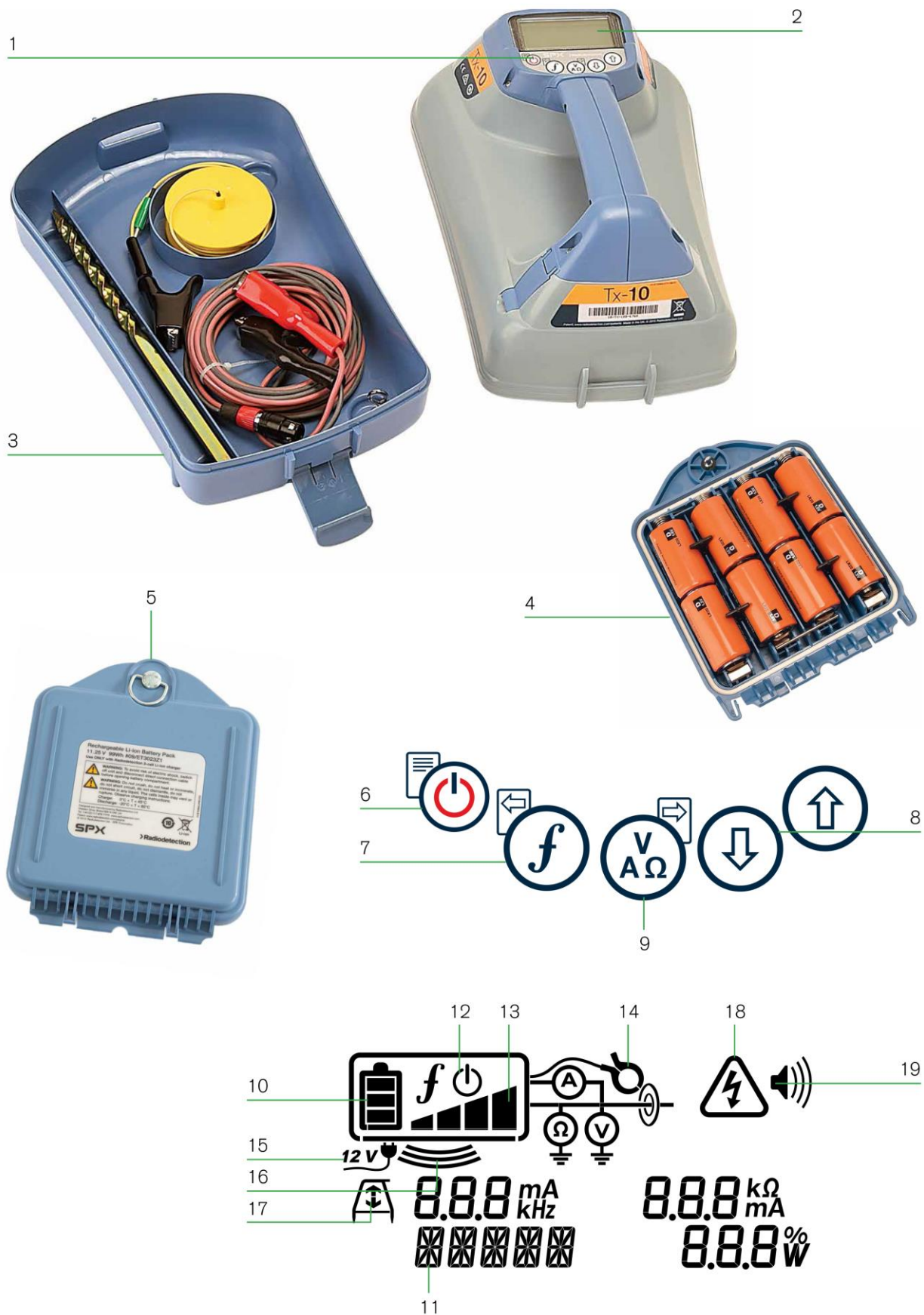
Figure 3.2 Tx Transmitter
