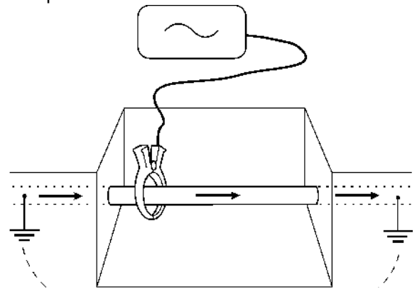
Figures 8.5 – 8.6: Connecting transmitter clamps
