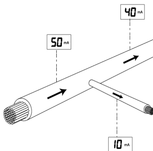
Figure 6.3 Current readings
